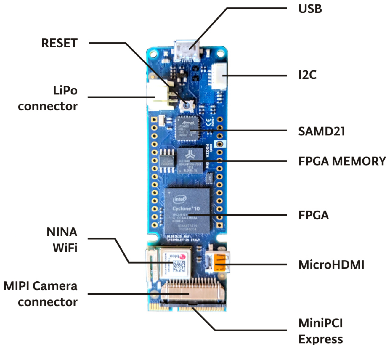
Board Overview
